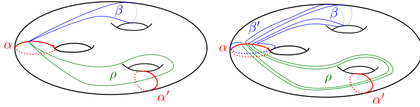
FIGURE 2. The construction in the proof of Lemma 6.7. The left figure shows the setup; the right one the curve constructed in the proof
