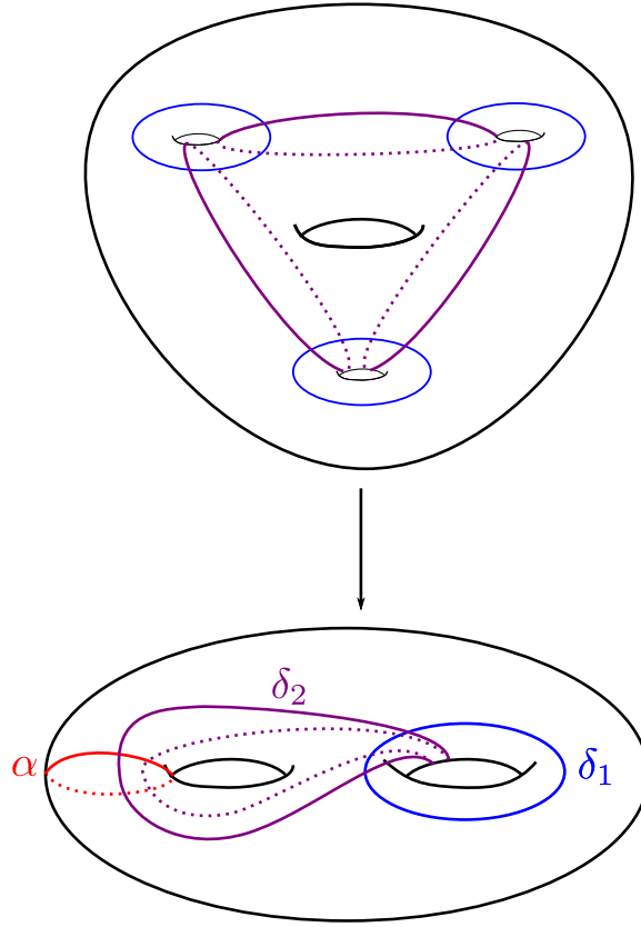
FIGURE 1. A 3-fold cover inducing odd intersections of meridians. The handlebody for the bottom surface is the “outside” handlebody of the standard Heegaard splitting of S^3 : curves are meridians if they can be contracted in the non-compact region of the page bounded by the surface.
