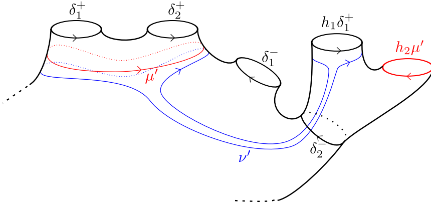
FIGURE 4. The construction in the proof of Lemma 6.11.
