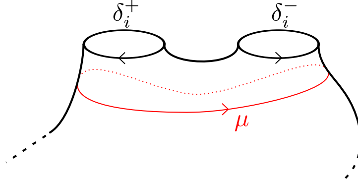
FIGURE 3. The construction in the proof of Lemma 6.10.
