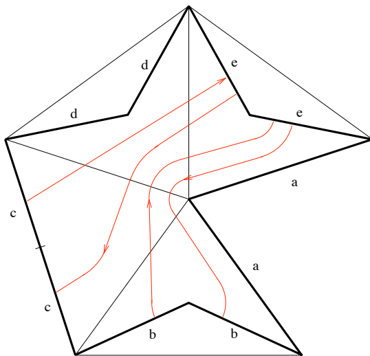
Figure 5: A generalized splittable curve
