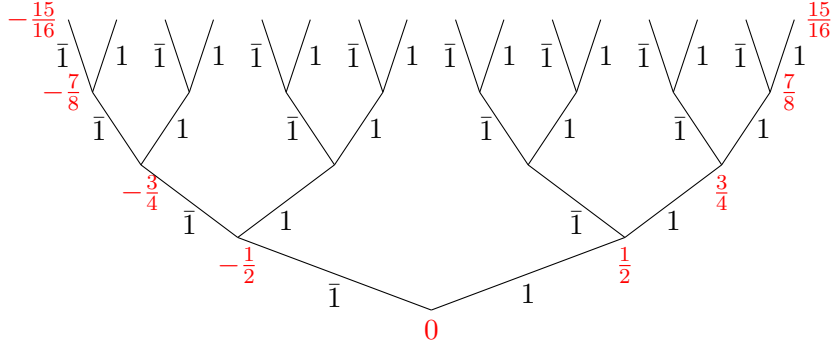
FIGURE 1. Dyadic rationals.
