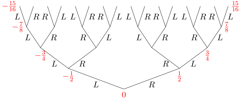
FIGURE 2. Gray code.
