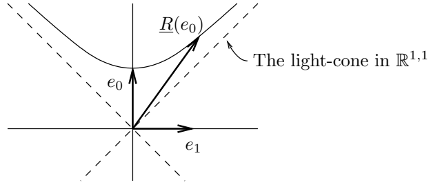
Figure 6.1: A Lorentz-boosted vector \underline{R}(e_0) , where R = \pm e^{\alpha I/2} and \alpha > 0 .
