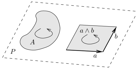
Figure 1.2: A 2-blade A represented by an outer product a \wedge b .
