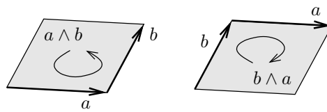
Figure 1.3: Geometric interpretation of b \wedge a = -a \wedge b .
