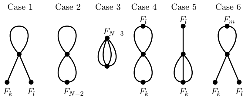
Figure 1: The six possibilities for the (quotient graph of groups of) the boundary splitting for spheres \sigma and \tau that intersect in a single circle. The splittings \sigma and \tau give refinements at the unlabelled vertex in each case, which has trivial stabilizer.
