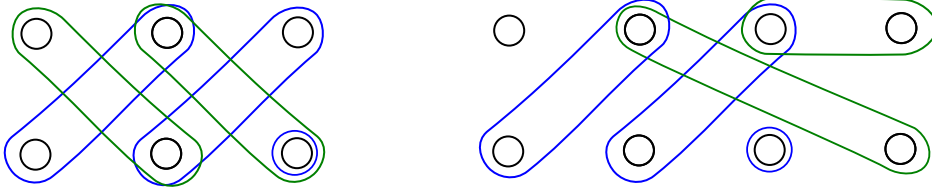
Figure 4: The proof of Lemma 3.16 in the case of N = 3 (on the left) and N = 4 (on the right). In each case, the spheres \sigma_1, \sigma_2 , and \sigma_3 are given in blue and the spheres \tau_1 and \tau_2 are given in green.
