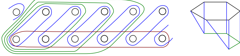
Figure 3: On the left is a description of the blow-up used in Lemma 3.13 when N = 6 in terms of spheres. The 12 black circles correspond to each side of the six spheres forming a rose, with x_i^+ and x_i^- pictured vertically. The blue spheres correspond to the partitions \mathcal{P}^i and the green spheres correspond to the partitions \mathcal{Q}^i . The sphere \tau is depicted in red. On the right is the graph given by the blow-up S \cup \Sigma .
