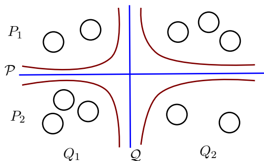
Figure 2: Crossing ideal edges \mathcal{P} and \mathcal{Q} are given as blue lines, with the associated boundary spheres shown in red.
