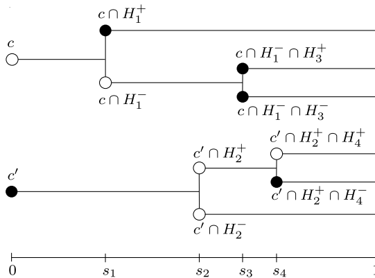
FIG. 1. Representation of a two-coloured branching tessellation in a finite window with initial tessellation T_0 = \{c, c'\} . The cells living at a time s constitute a tessellation T_s . At each time s_i , a cell that lives up to this moment is selected and cut in two by a bi-coloured hyperplane H_i , which impresses its colours onto the cell's pieces.
