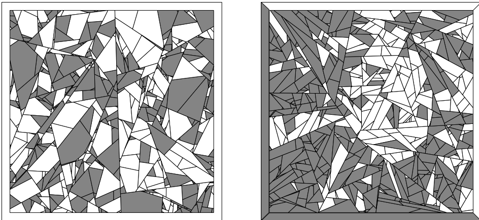
FIG. 2. Simulations of two BRTs with isotropic selection of lines, two colours and the full window as single initial cell. Left: A STIT tessellation; colours are chosen at random. Right: Colour mutation and size balancing as in Example 2.10, but without aging. Here, \varepsilon = 0.025 , \beta(\mathbf{s}) = (1 + \mathbf{s})/2 and a mixed boundary condition as indicated.
